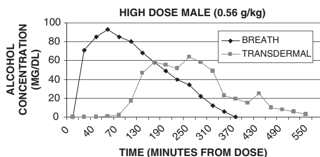
Fig. 2. Transdermal and breath alcohol concentration curve for one participant in the high-dose group in the laboratory study.
